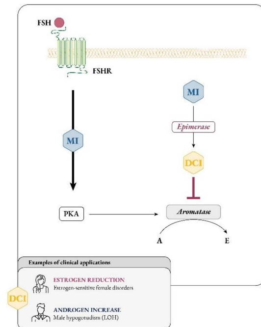
Figure 4. Myo-inositol and D-chiro-inositol affect aromatase activity in an opposite manner. Abbreviations: FSH, follicular stimulating hormone; FSHR, FSH receptor; MI, myo-inositol; DCI, D-chiro-inositol; PKA, protein kinase A; A, androgen; E, estrogen; LOH, late onset hypogonadism.
